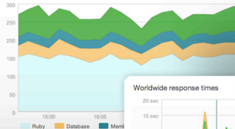
Average response time, broken down by tier (ms)
