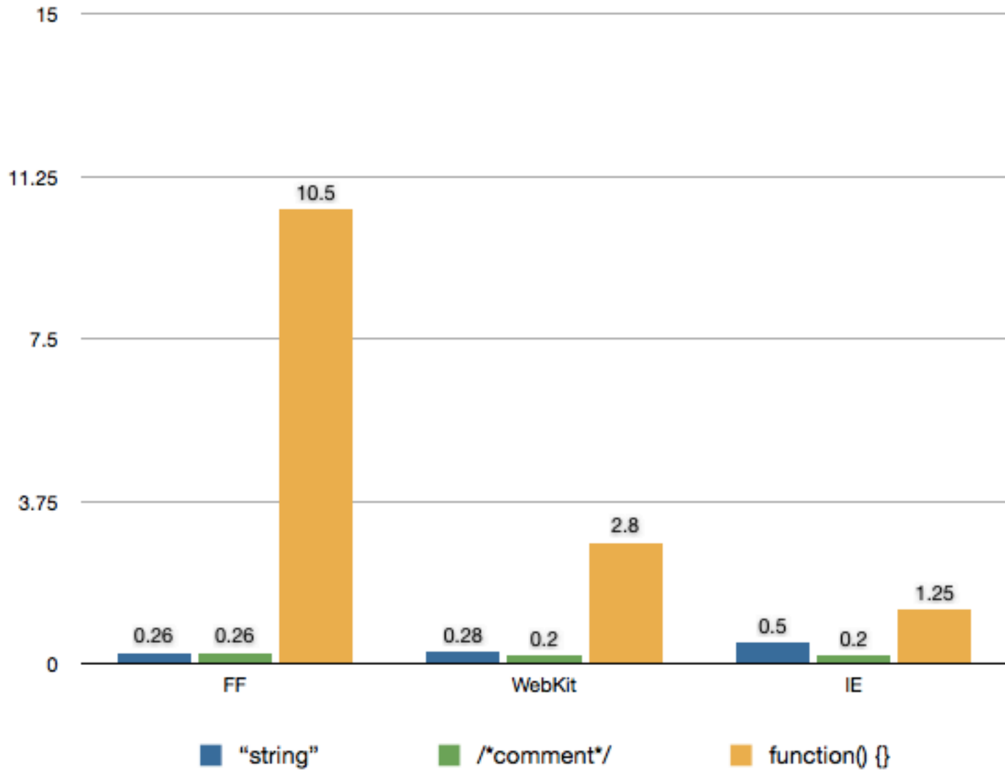
eval() time for code as:
